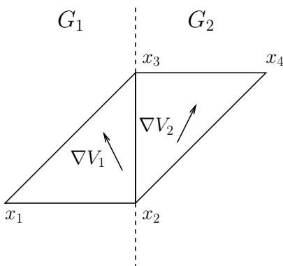
FIGURE 1. Gradient conditions (13) for two adjacent simplices
