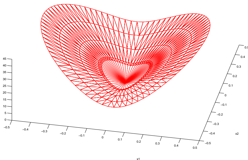
FIGURE 3. Lyapunov function for Example 5.2
